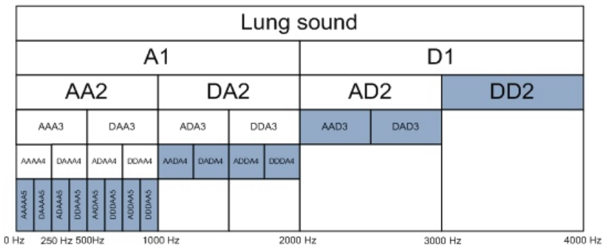
Fig. 6. Sub-band used in WPD scheme.
