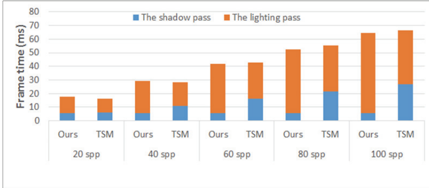
Fig. 11. Timing for each step of our algorithm and TSM when rendering the scene in Fig. 9.
