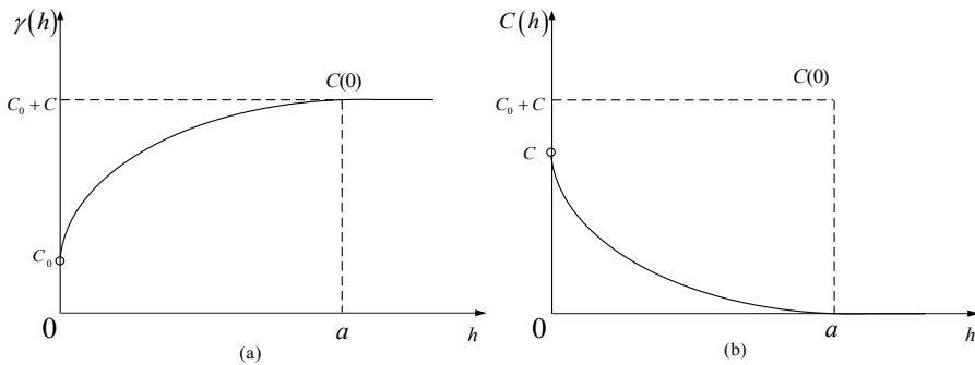
Fig. 1. Variation function graph: (a) variation function \gamma(h) and (b) corresponding covariance function graph.
