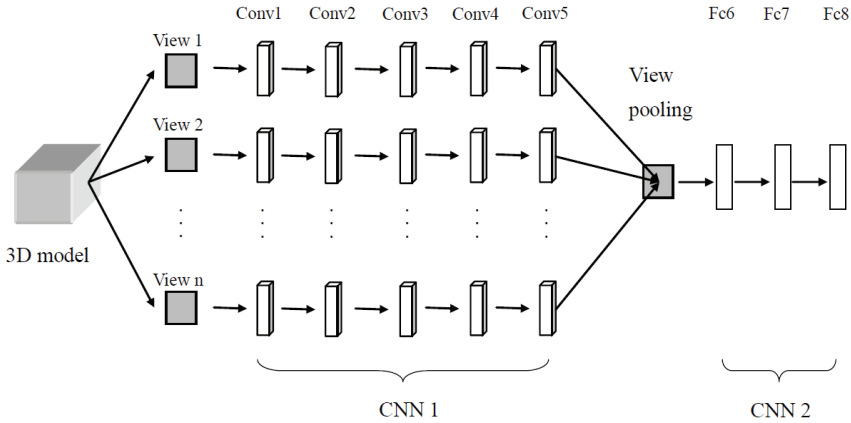
Fig. 1. Architecture of MVCNN model.
