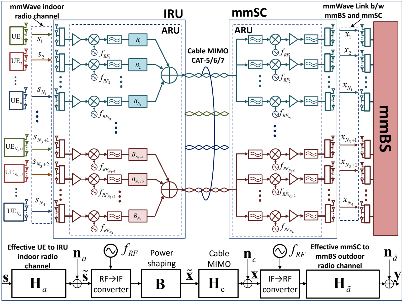
Fig. 5. System model for uplink transmission via mmWoC architecture.
