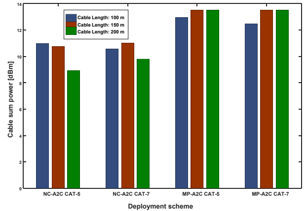
Fig. 8. The sum power (in dBm) on the cable in all the considered scenarios.
