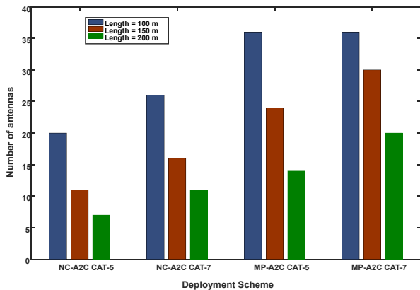
Fig. 7. The number of antennas supported in all the considered scenarios.
