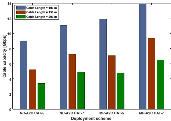
Fig. 6. Cable capacity (in Gbps) achieved by all the considered scenarios.
