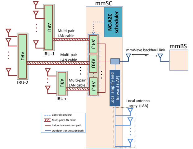
Fig. 3. Functional diagram of the proposed mmWoC based access network architecture for indoor coverage.
