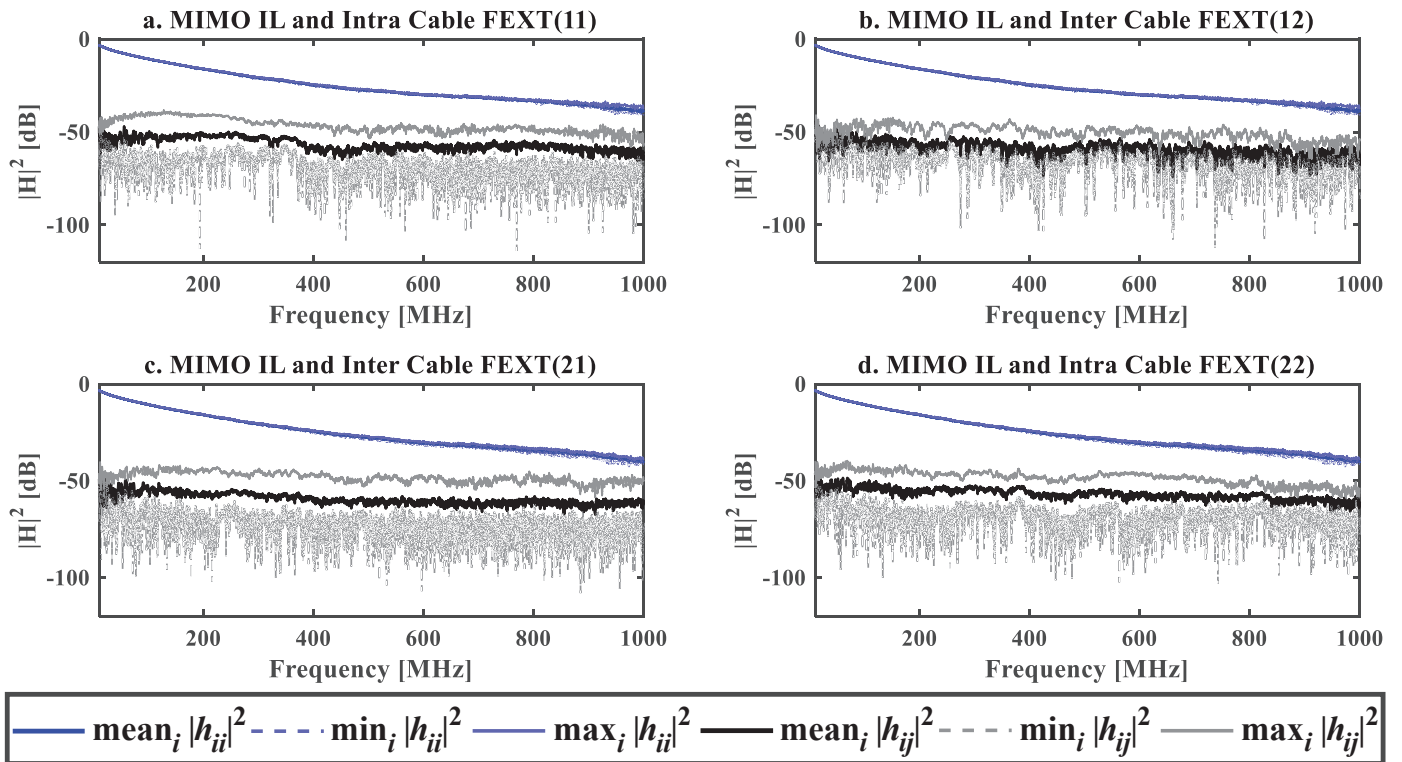
Fig. 10. IL Vs FEXT for Cable binder with 2 CAT-5 LAN cables of 50m length.
