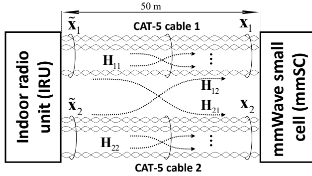
Fig. 9. Cable binder with 2 CAT-5 LAN cables connected between IRU and mmSC.
