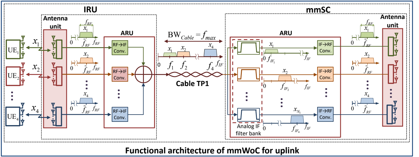
Fig. 4. Functional architecture of ARU at IRU and mmSC for uplink.
