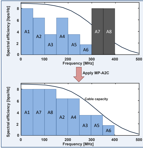
Fig. 2. An example of MP-A2C scheduler operation for 8 antenna signals on a single twisted pair.
