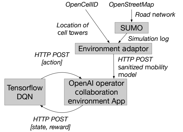
Fig. 3. Simulation environment.
