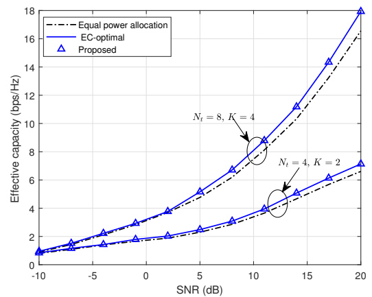
Fig. 6. Effective capacity with regard to SNR for different value of N_t and K .
