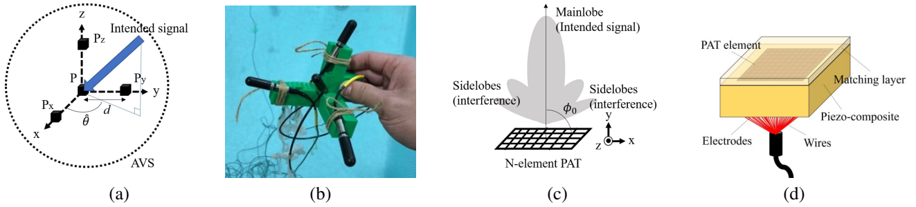
Fig. 2. (a) 4-element acoustic vector sensor (AVS), where \hat{\theta} is the estimated angle of direction on the x - y plane; (b) Photo of the proposed acoustic vector sensor, which is composed of 4 omni-directional hydrophones; (c) N -element uniform rectangular phased array BF, where \phi_0 shows the steering angle; and (d) 3-D PAT sample image, in which each PAT element has an independent electrode at the bottom connected with a wire to the controller.
