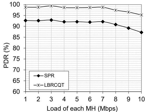
Fig. 9. Packet delivery ratio performances of SPR and LBRCQT in case of the variable traffic load.
